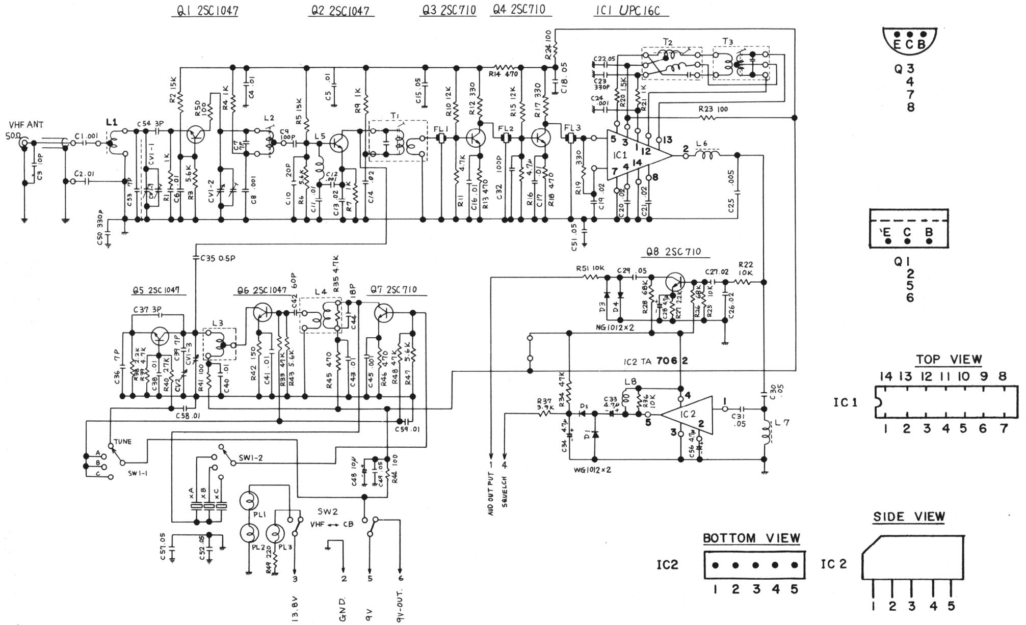
FIGURE 10, SCHEMATIC DIAGRAM, VHF/FM MONITOR, ISSUE D
