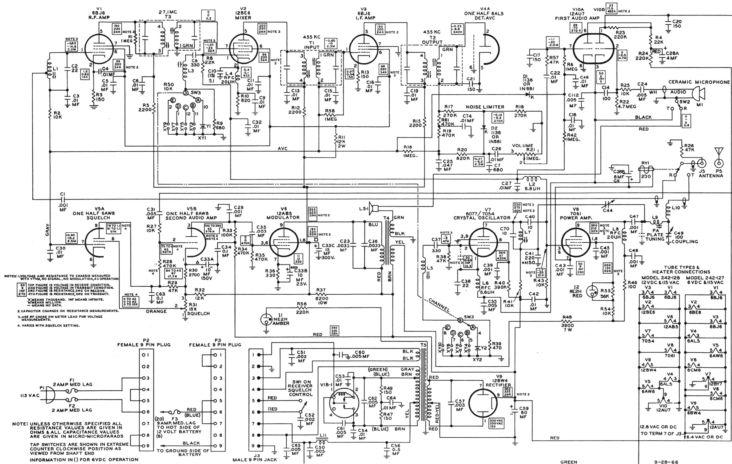
MESSENGER I SCHEMATIC MODELS 242-127 AND 242-128
