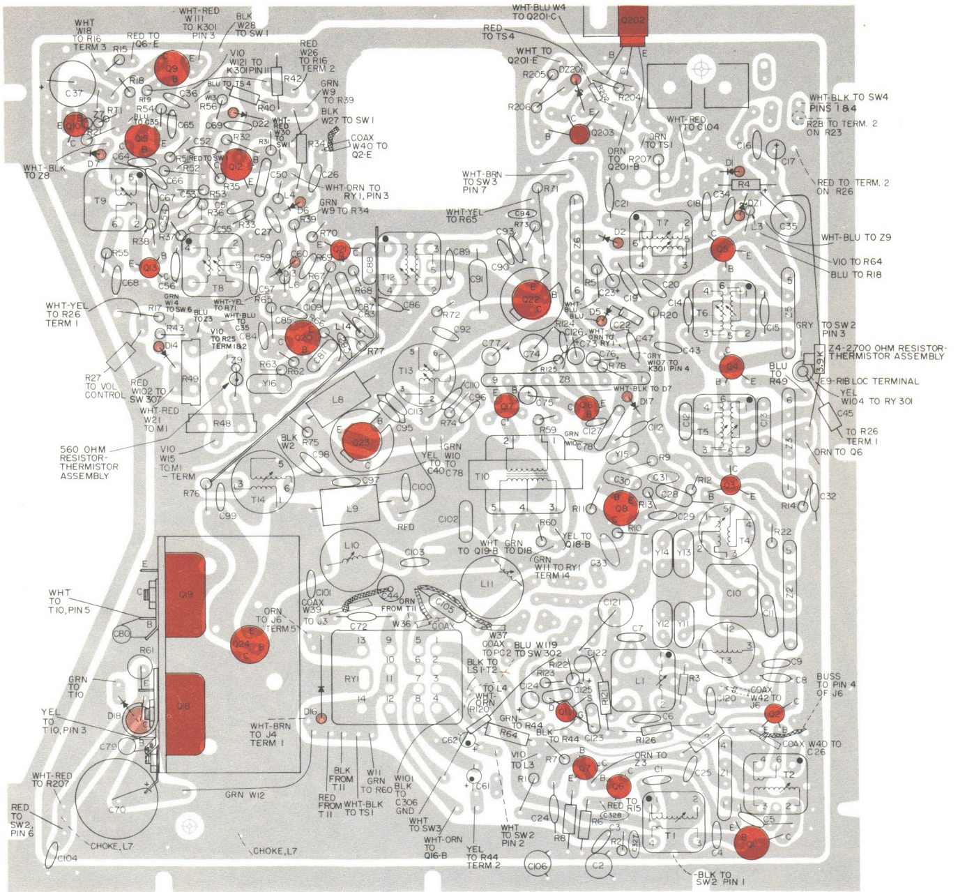
TRANSCIVER PRINTED CIRCUIT BOARD COMPONENTS LAYOUT (AS VIEWED FROM THE SOLDER SIDE OF THE BOARD)
