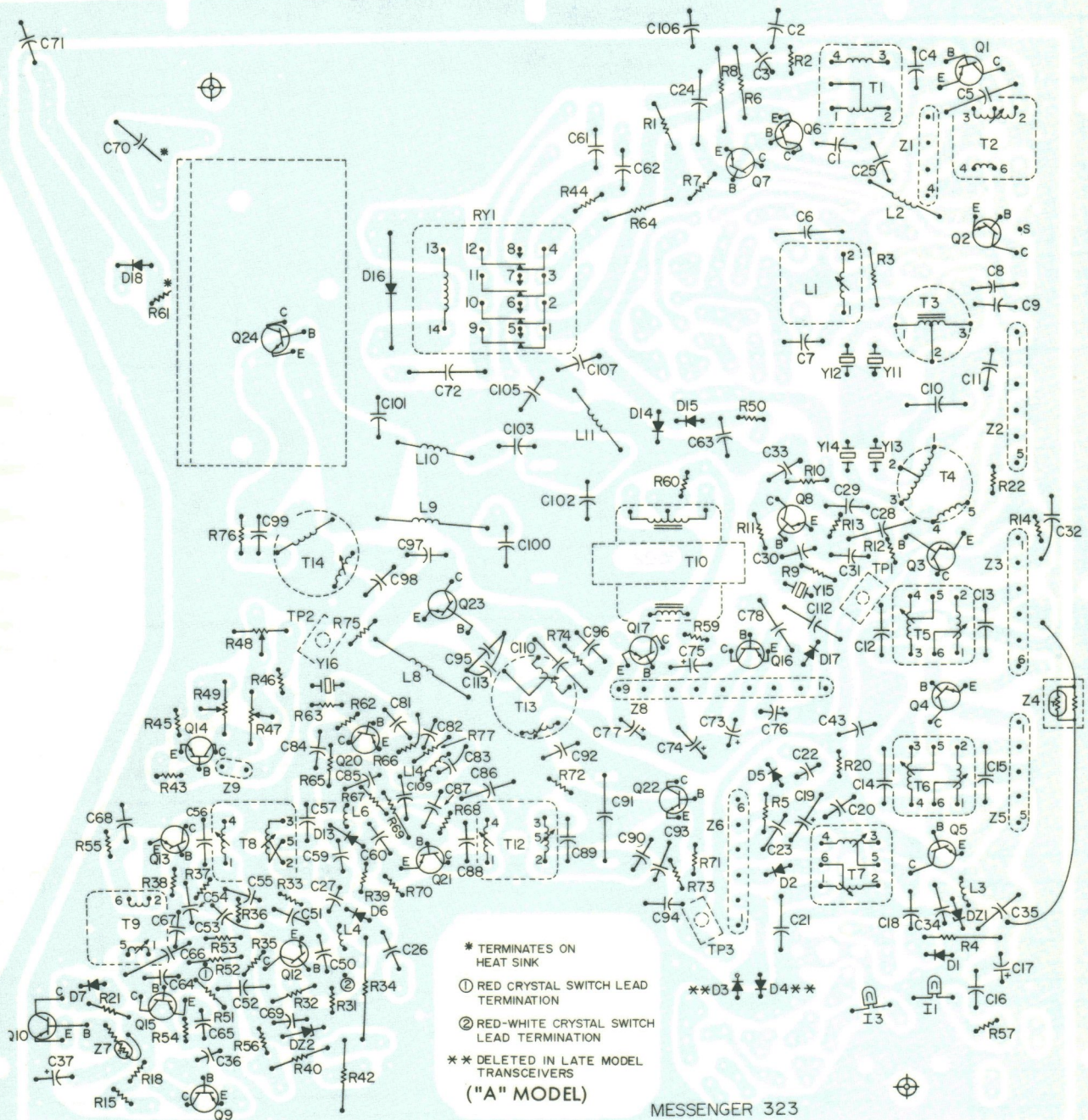
PRINTED CIRCUIT COMPONENTS LOCATION
