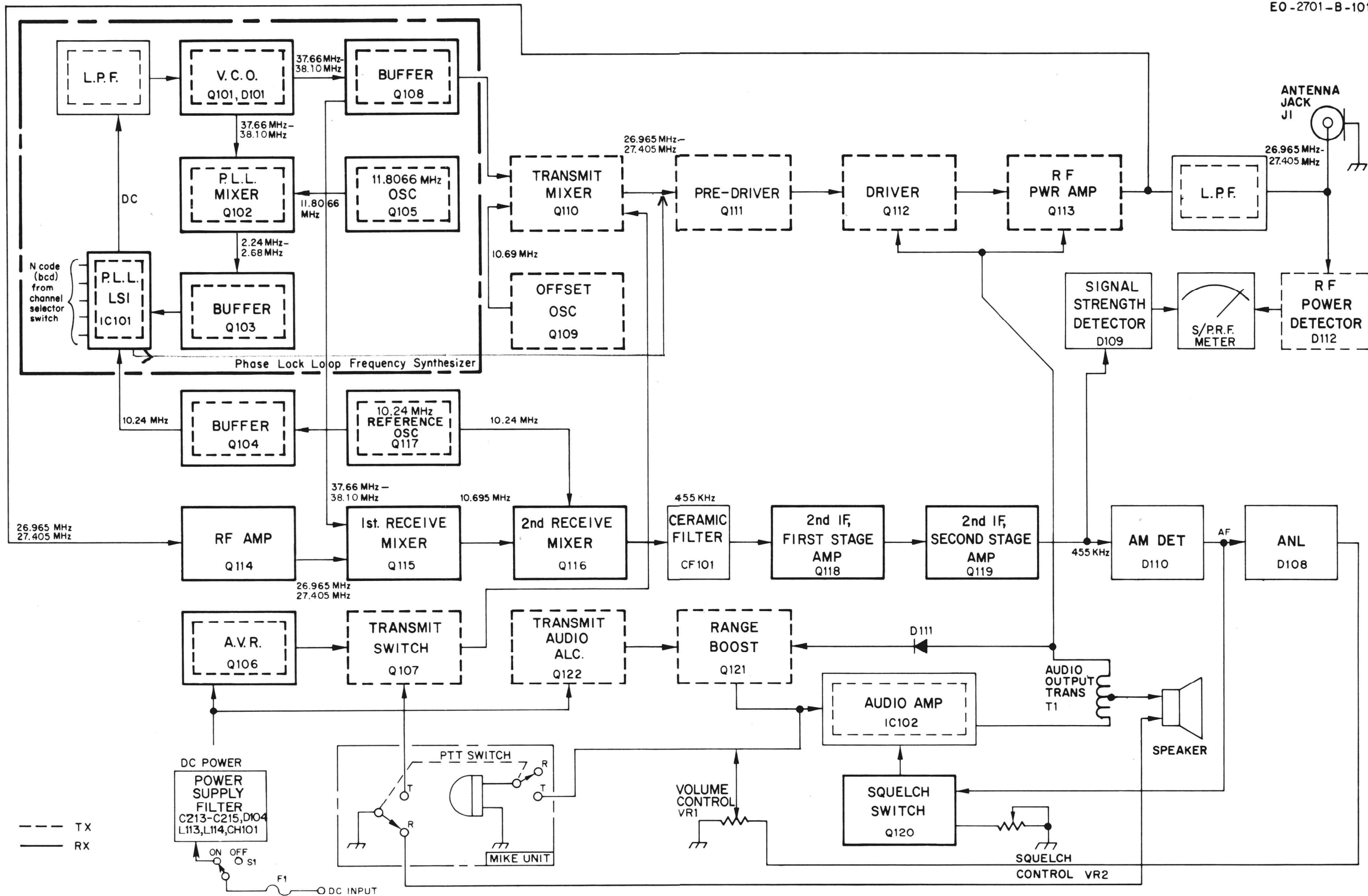
Figure 2-2. Block Diagram, Model 2701
