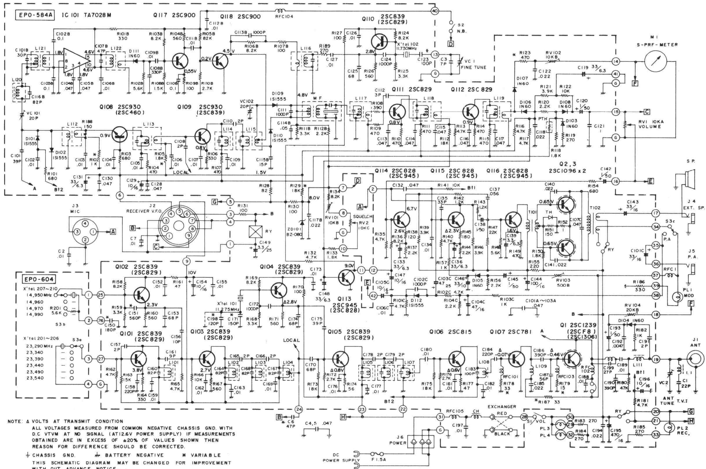
SCHEMATIC DIAGRAM HY - GAIN 672
