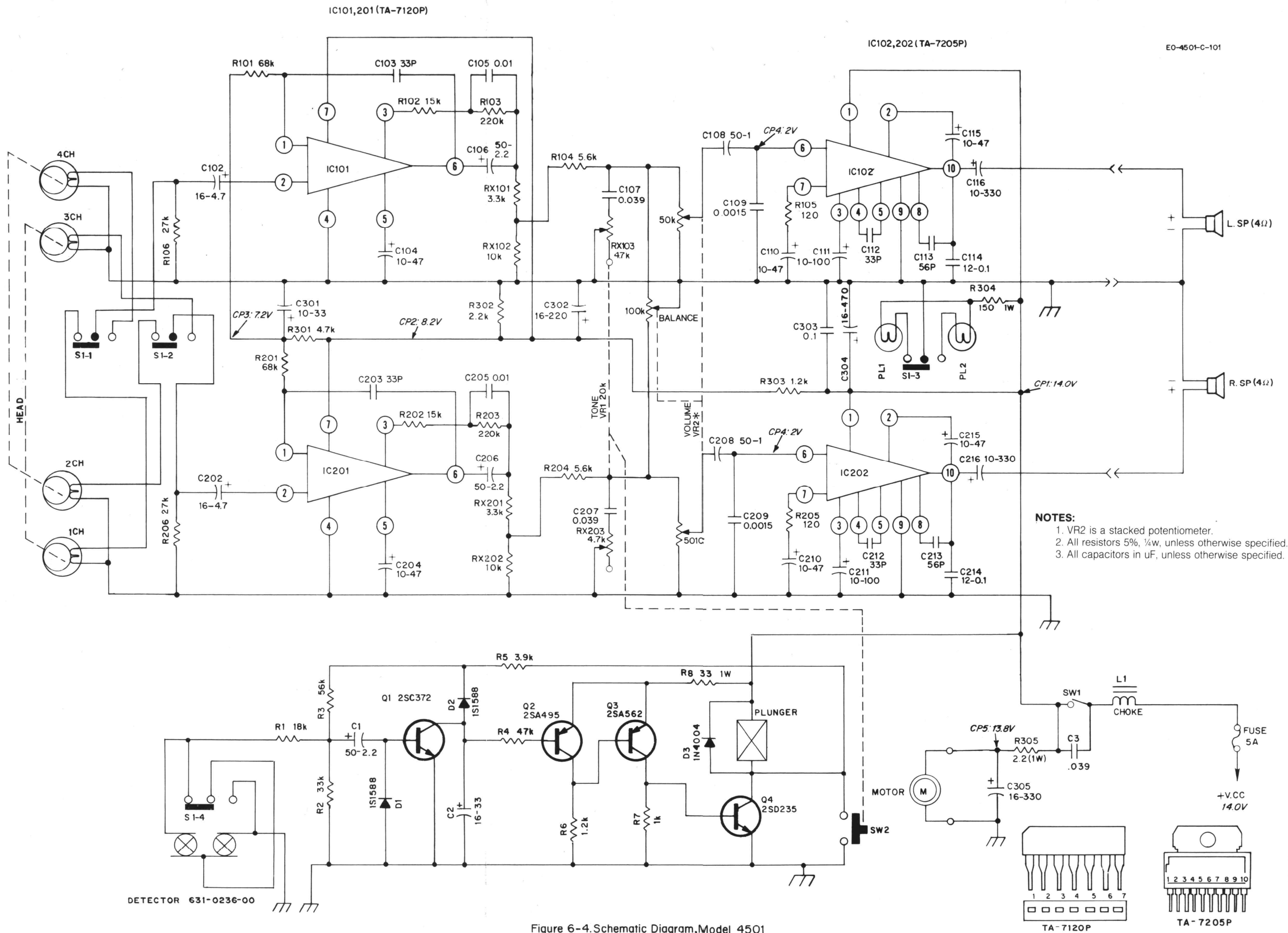
Figure 6-4. Schematic Diagram, Model 4501
