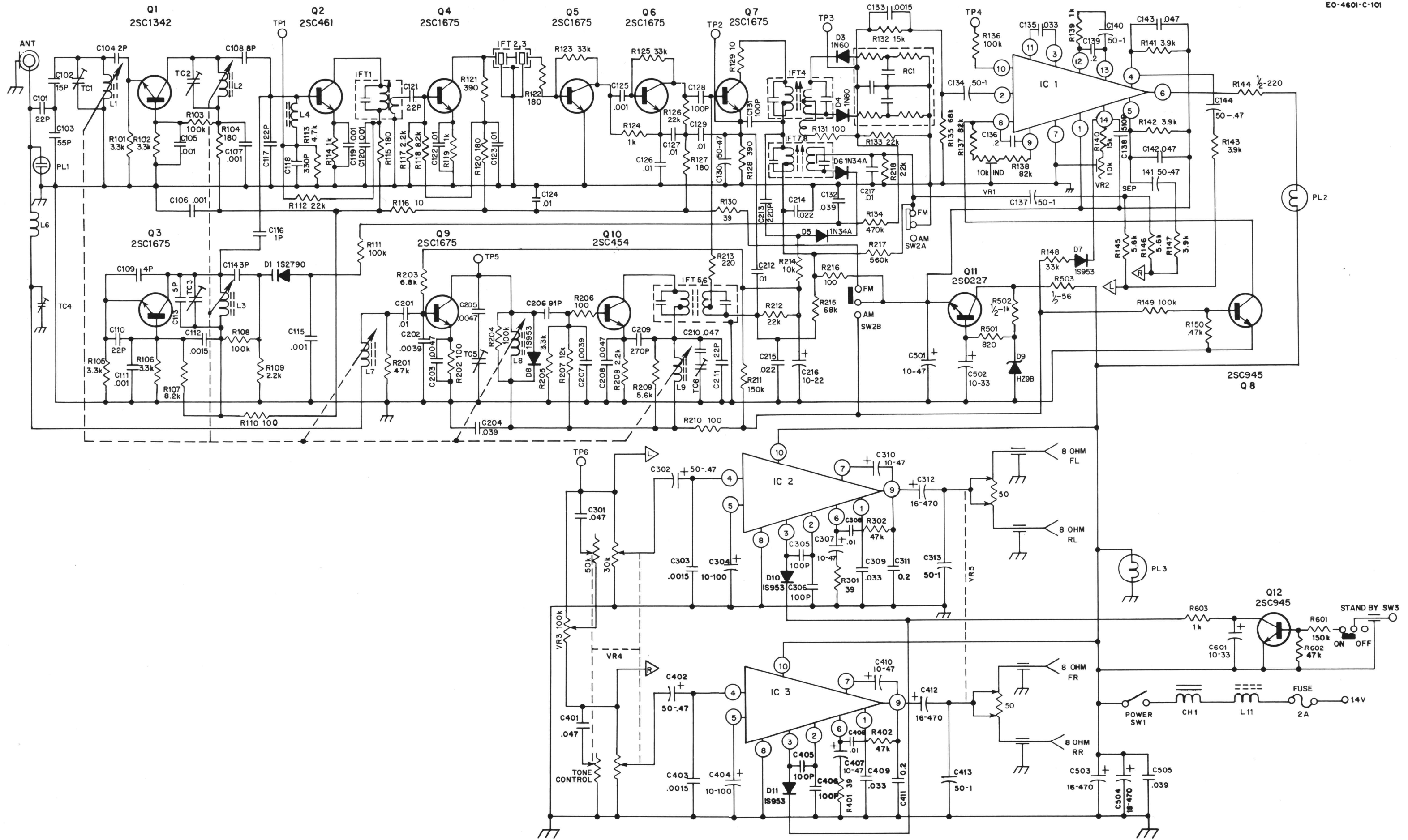
Figure 5-3. Schematic Diagram, Model 4601
