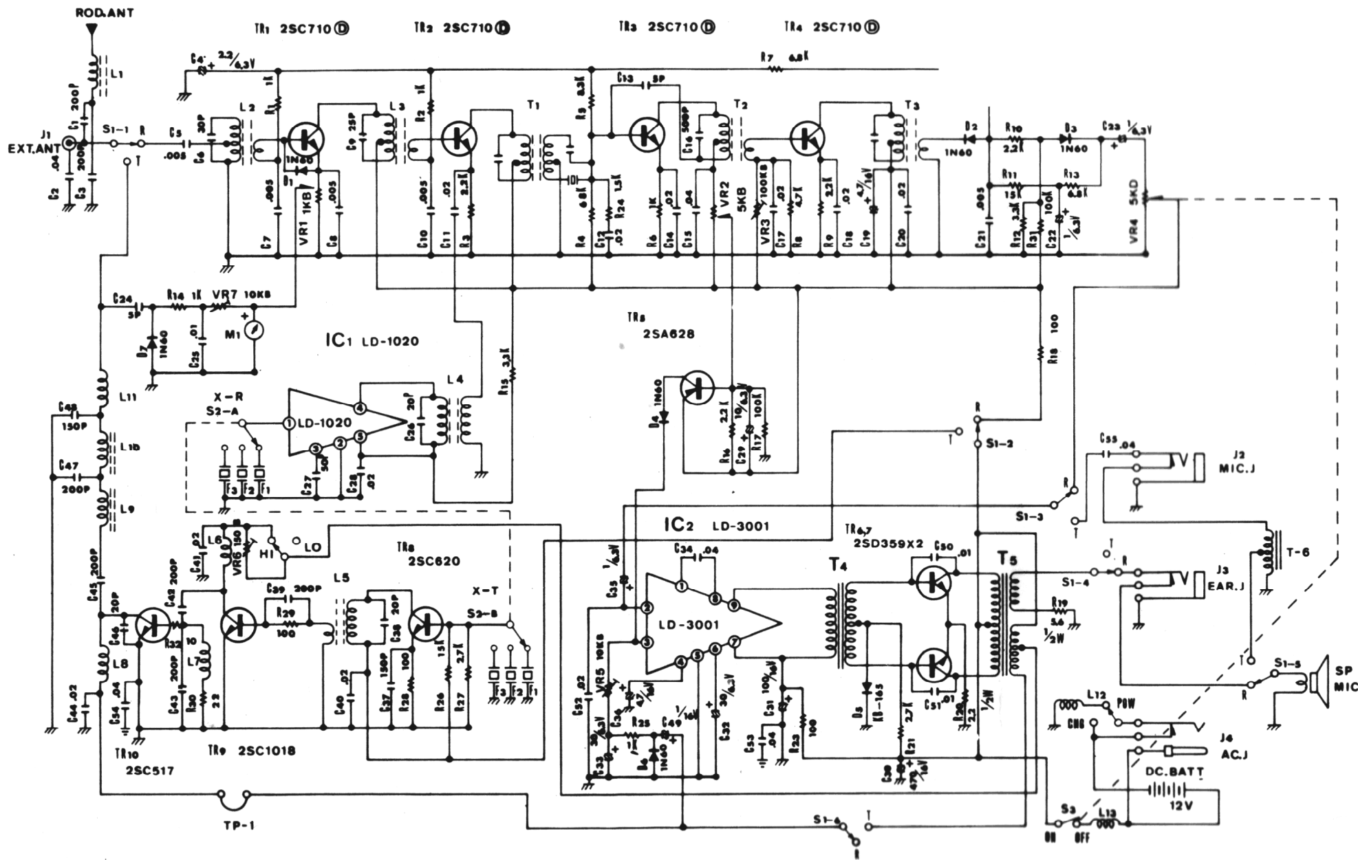
5W TRANSCEIVER SCHEMATIC DIAGRAM MODEL 13-785
