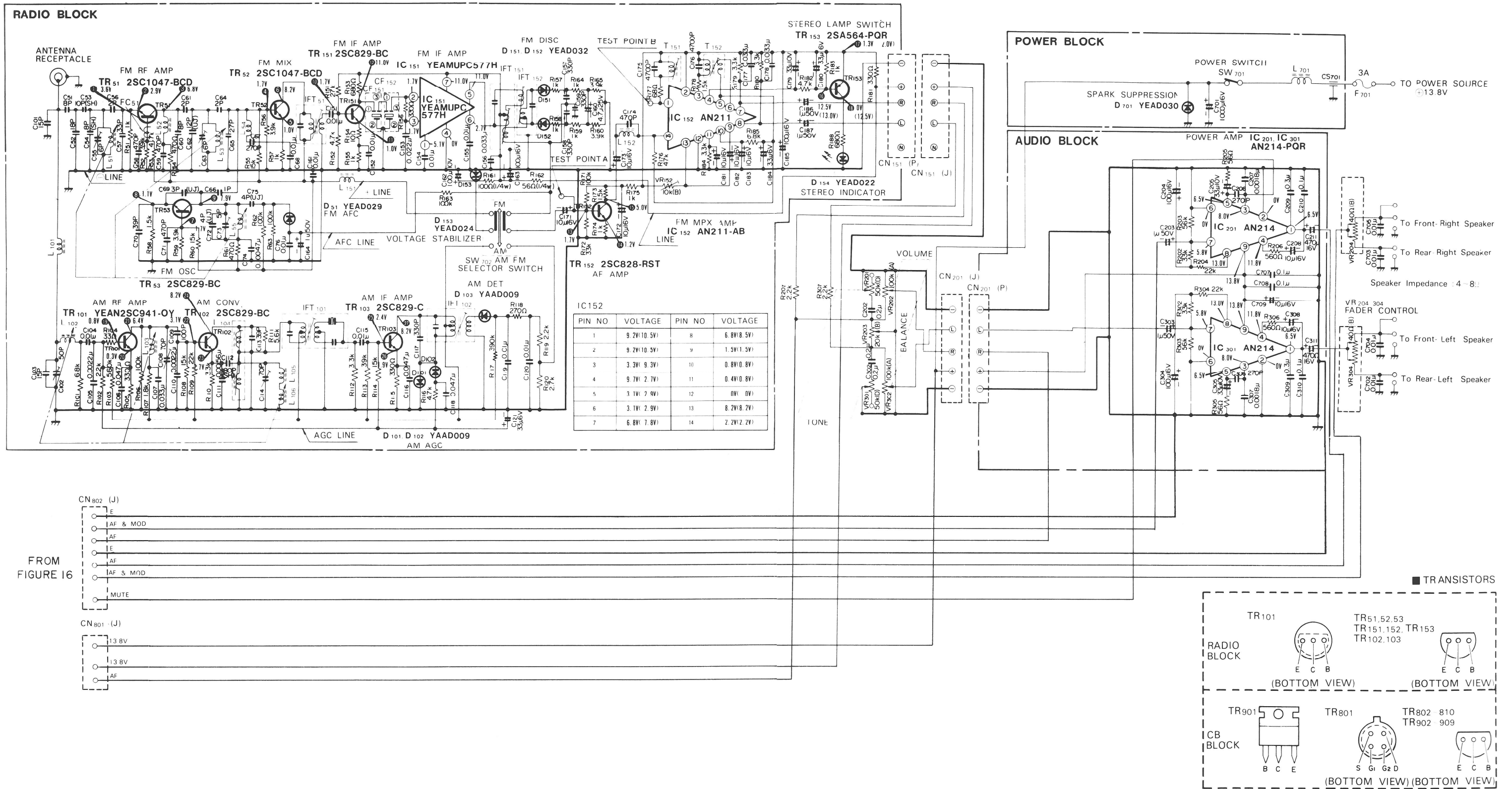
Figure 17. AM/FM/FM Stereo Radio, Audio, and Power Circuits, Schematic Diagram
