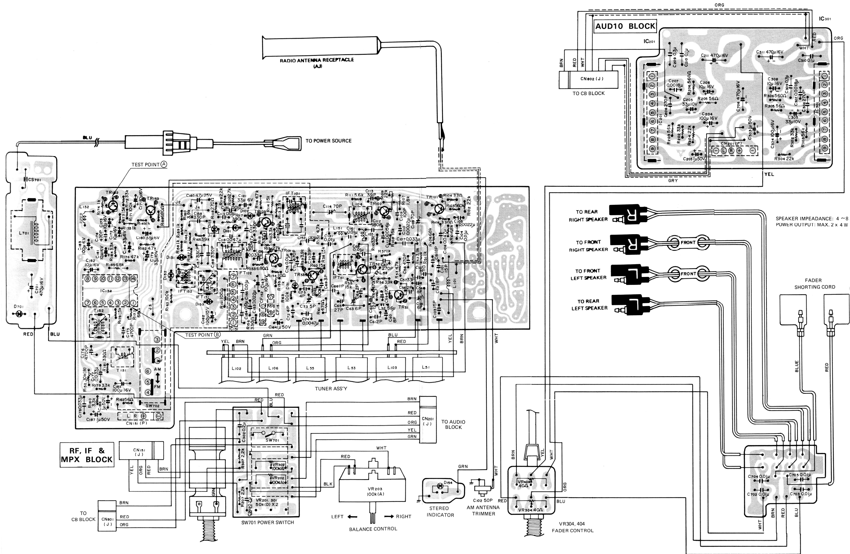
30 Figure 15. Printed Board – Radio Block – 14T405
