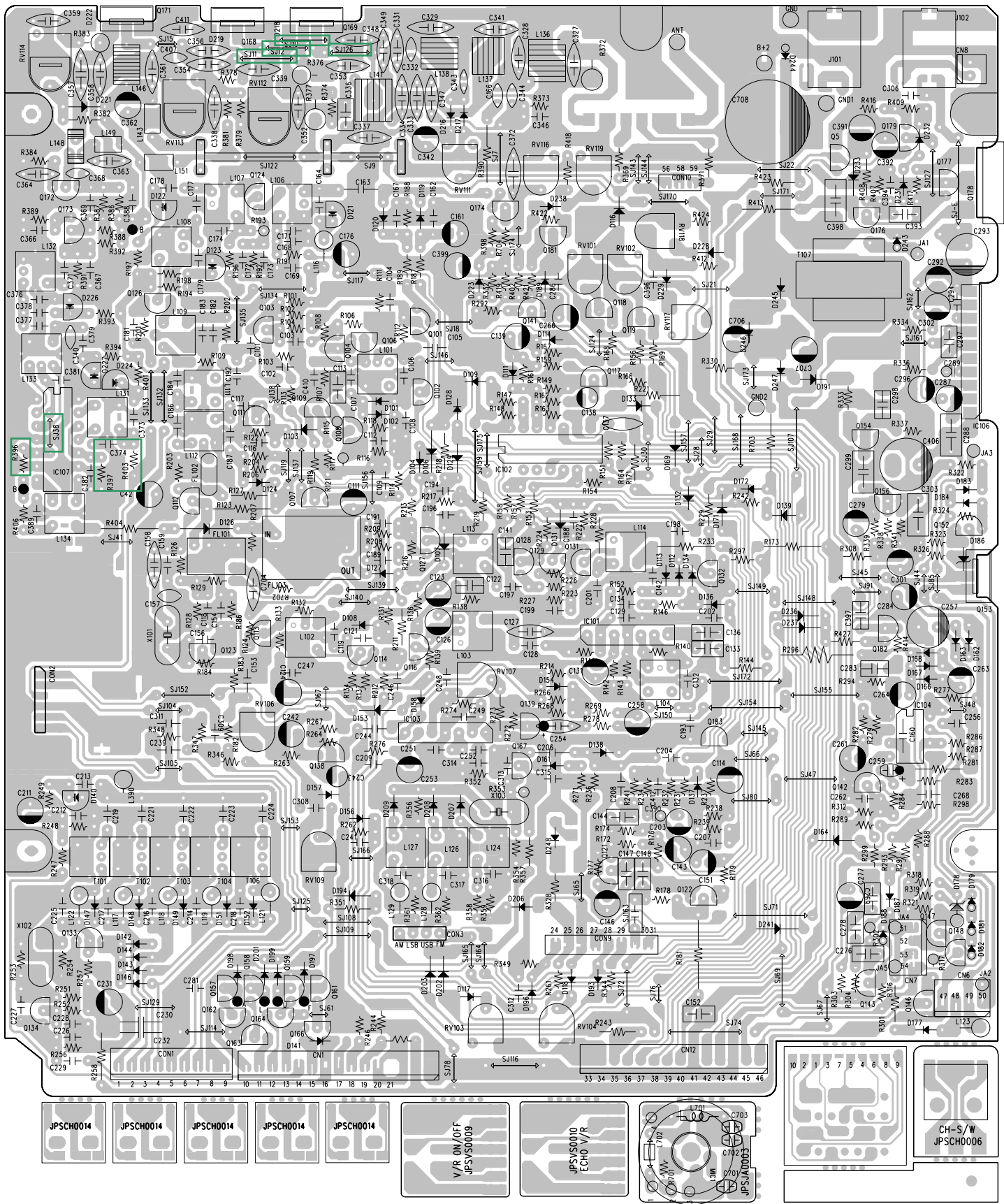
Magnum S45HP Main PCB Parts Layout
