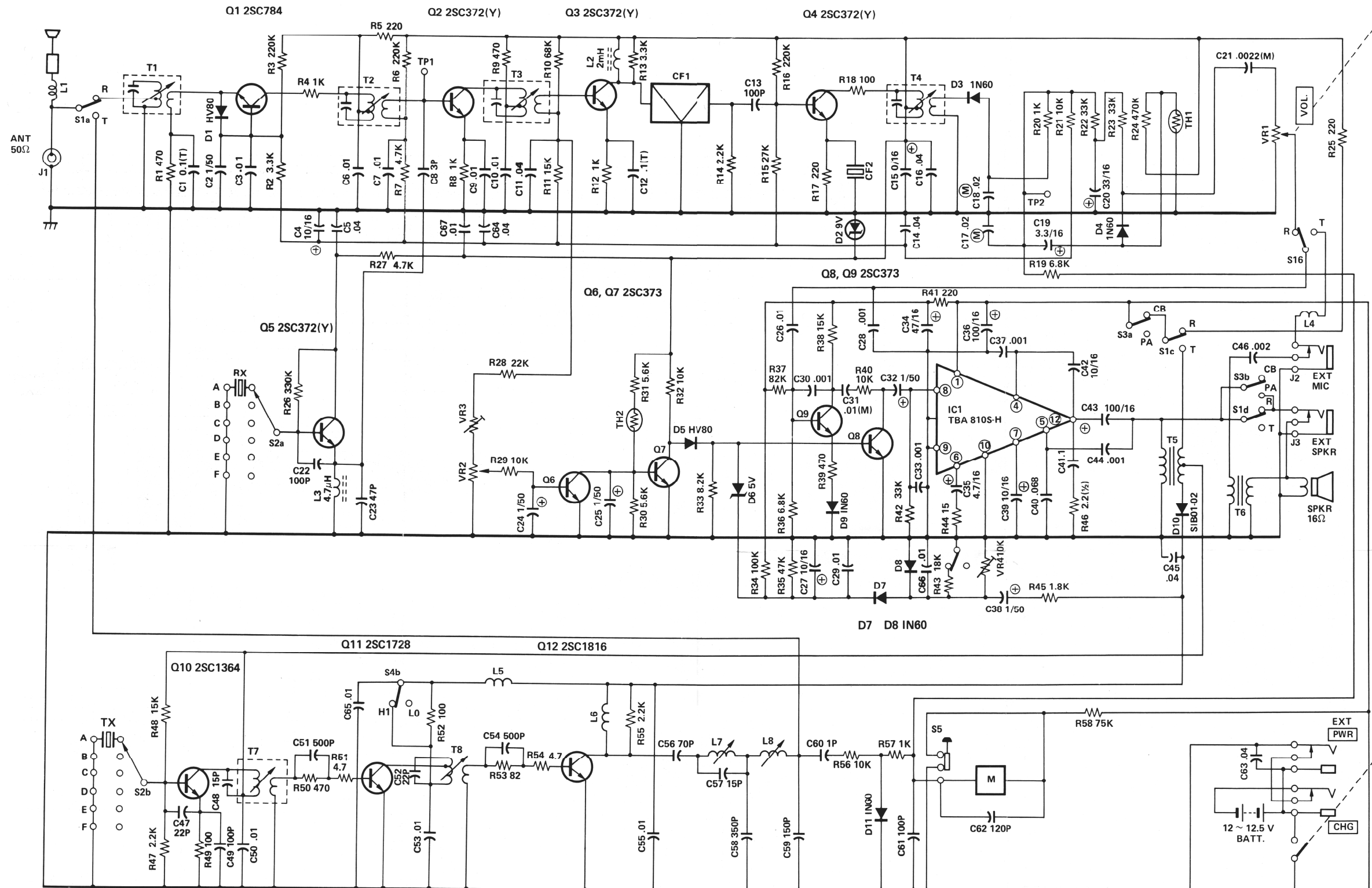
SBE 31 CB TRANSISTOR VOLTAGES (12.5V DC input)
