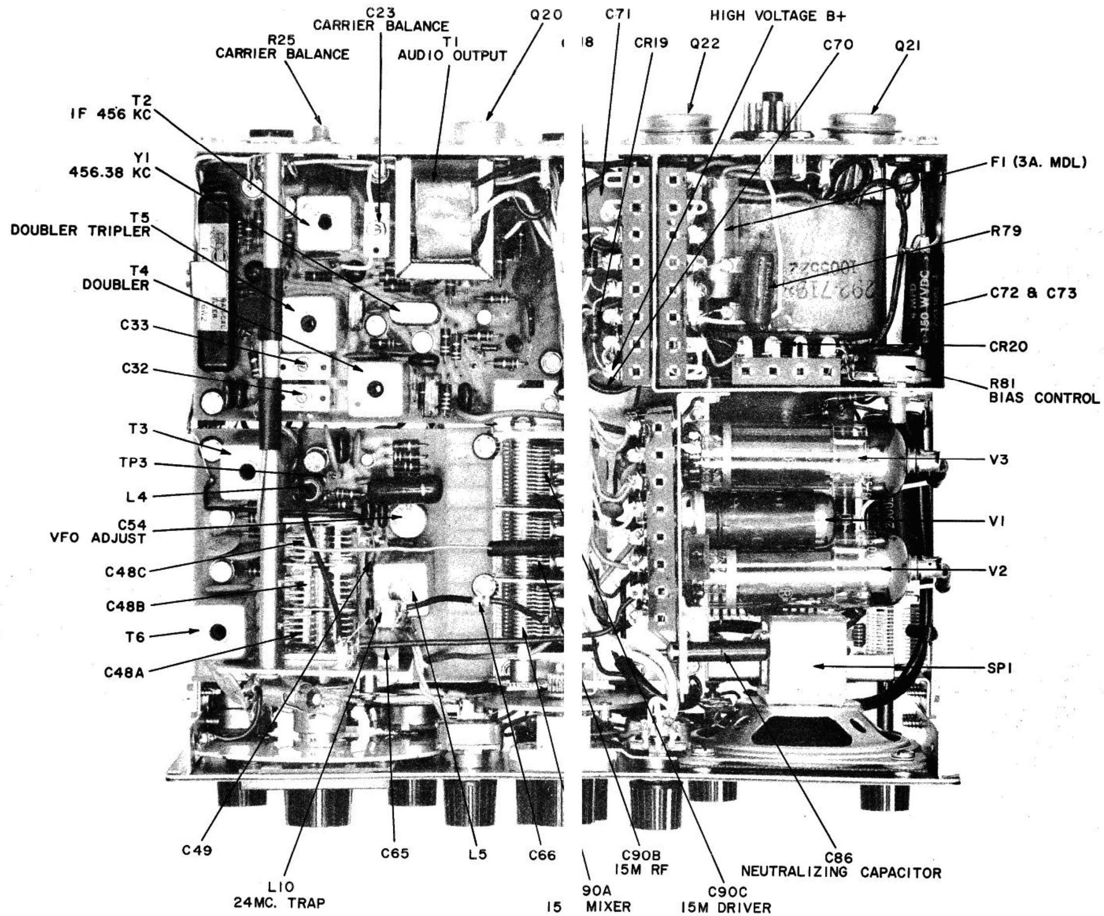
CHASSIS TOP VIEW
