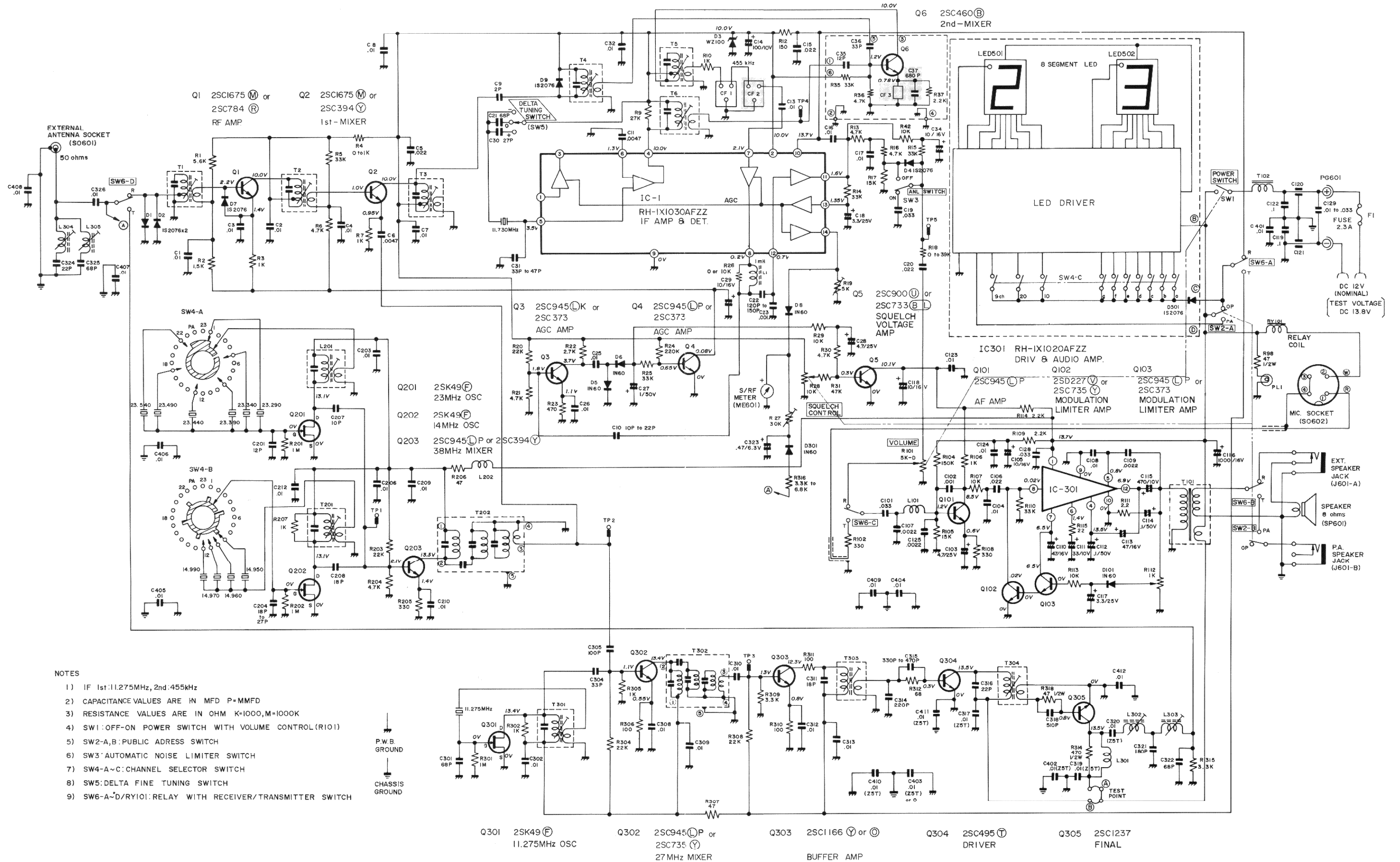
Figure 20 SCHEMATIC DIAGRAM (P.W.B. NO. F0485AF-4)
