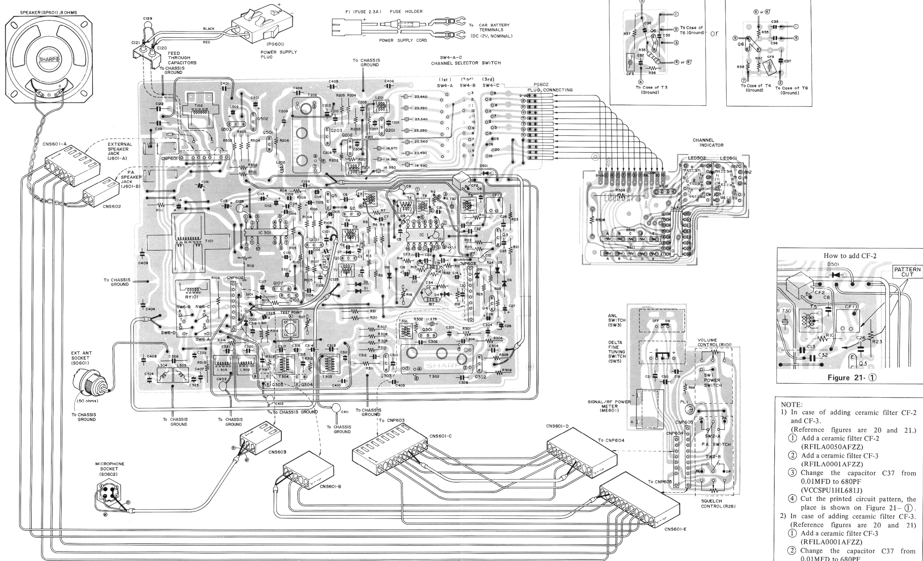
Figure 21 WIRING SIDE BOARD (P.W.B. NO. F0485AF-4)
