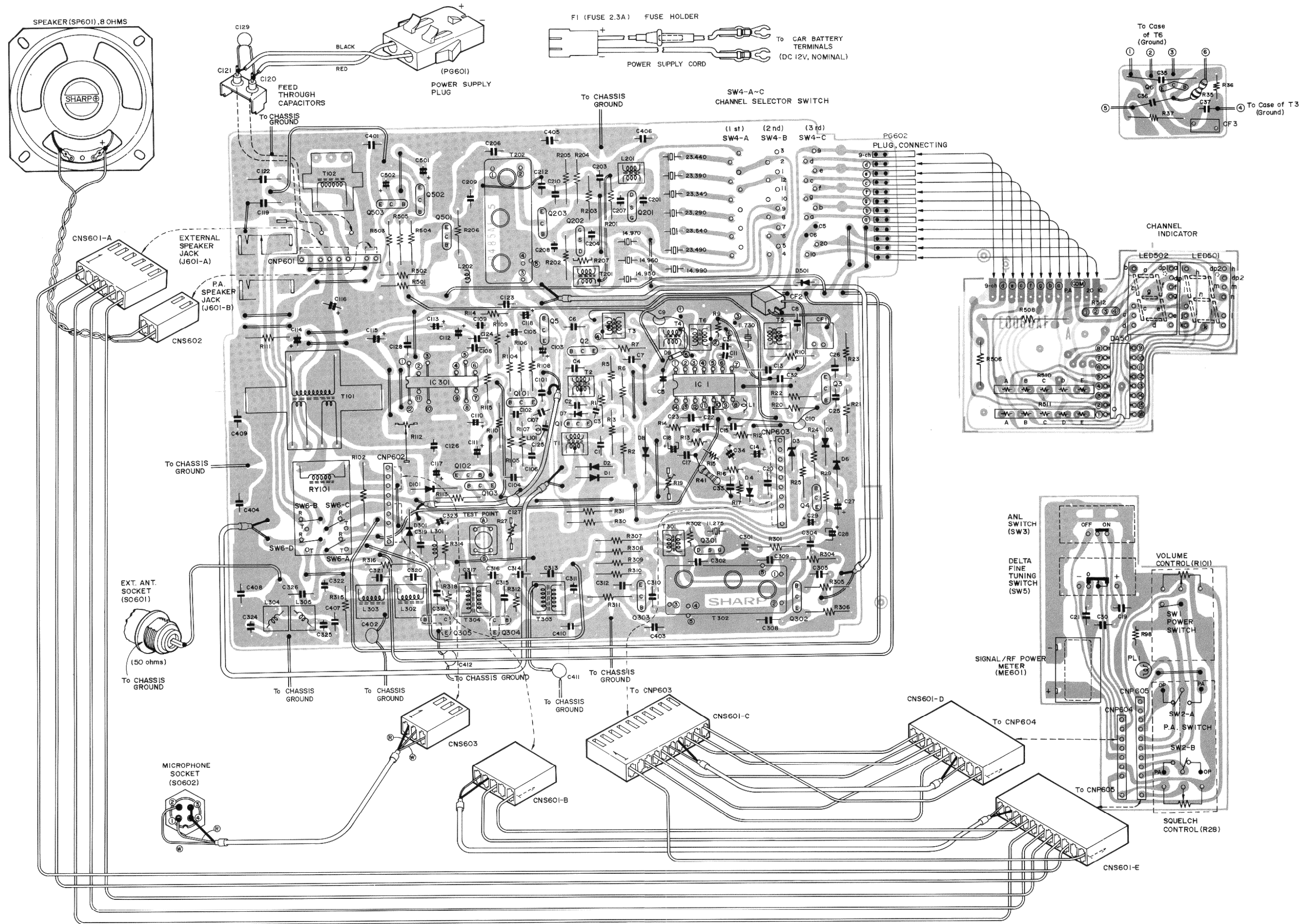
Figure 23 WIRING SIDE BOARD (P.W.B. NO. F0485AF-5)
